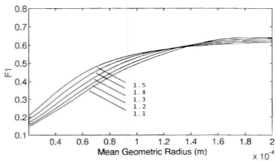
Figure 2.5 Response functions for 1.323 MHz and 5.292 MHz, assuming a lognormal particle size distribution, as a function of the particle mean geometric radius for values of \sigma_g = 1.1, 1.2, 1.3, 1.4, 1.5 .
